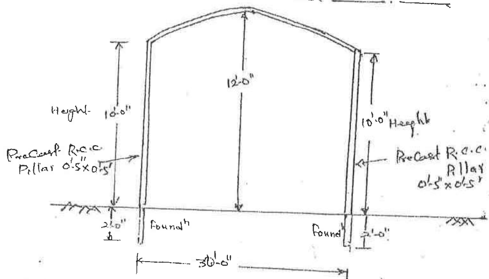
SIDE ELEVATION OF PROPOSED MASHROOM HUT AT DR. R.P.C.A.U. PUSA
