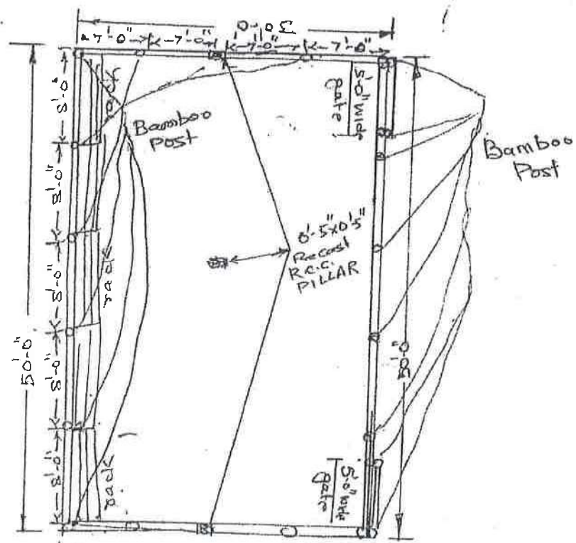
PLAN OF PROPOSED MASHROOM HUT AT DR. R.P.C.A.U. PUSA
